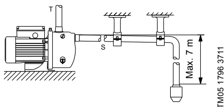
Fig. 2 Pipe connection
